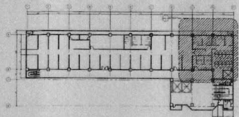
KEY PLAN SCALE: 1/200 MTS
